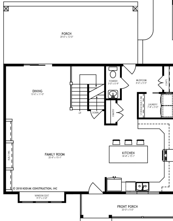
FIRST FLOOR PLAN AREA: 990 square feet
