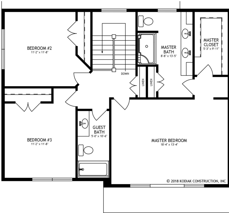
SECOND FLOOR PLAN AREA: 992 square feet
