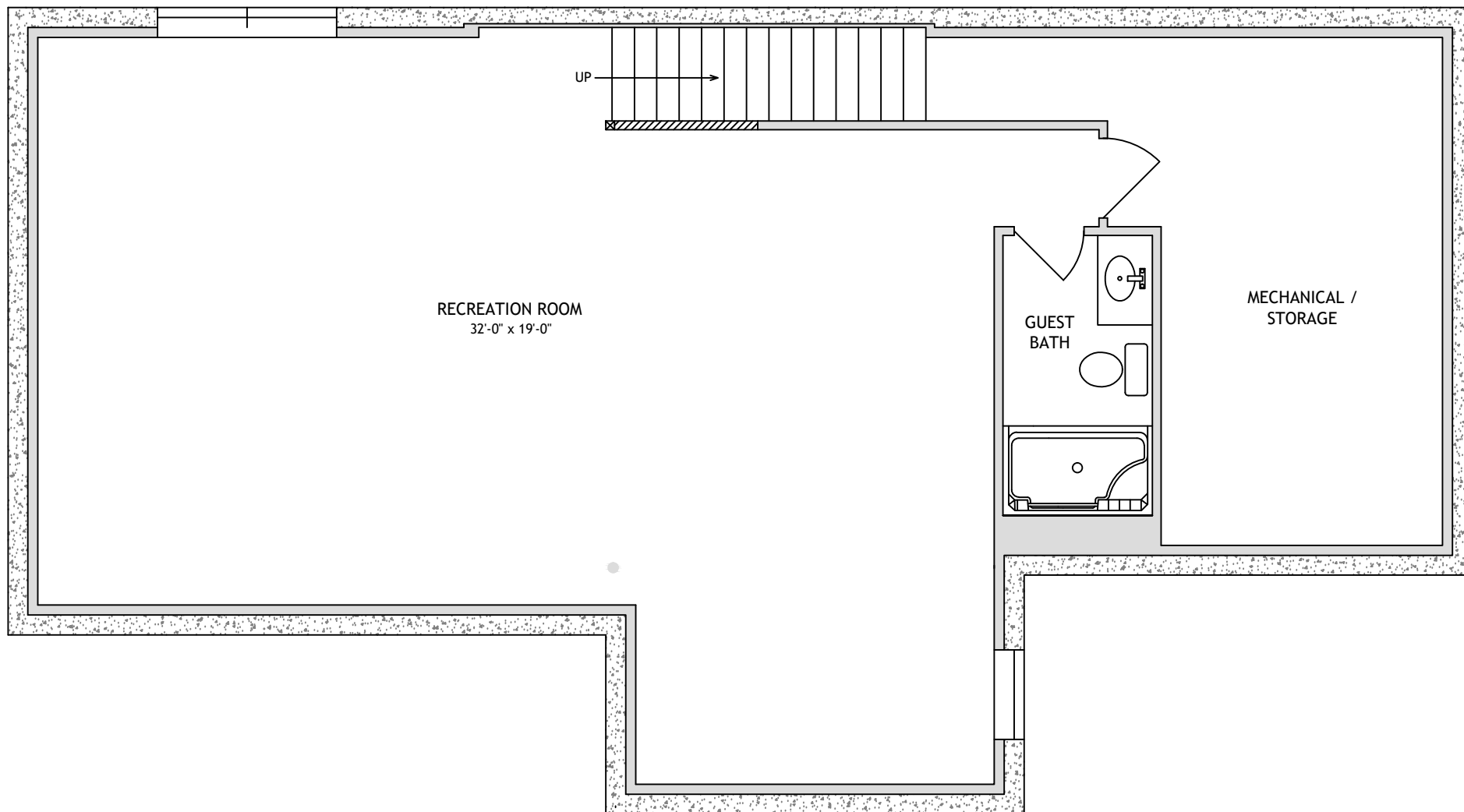
BASEMENT PLAN
